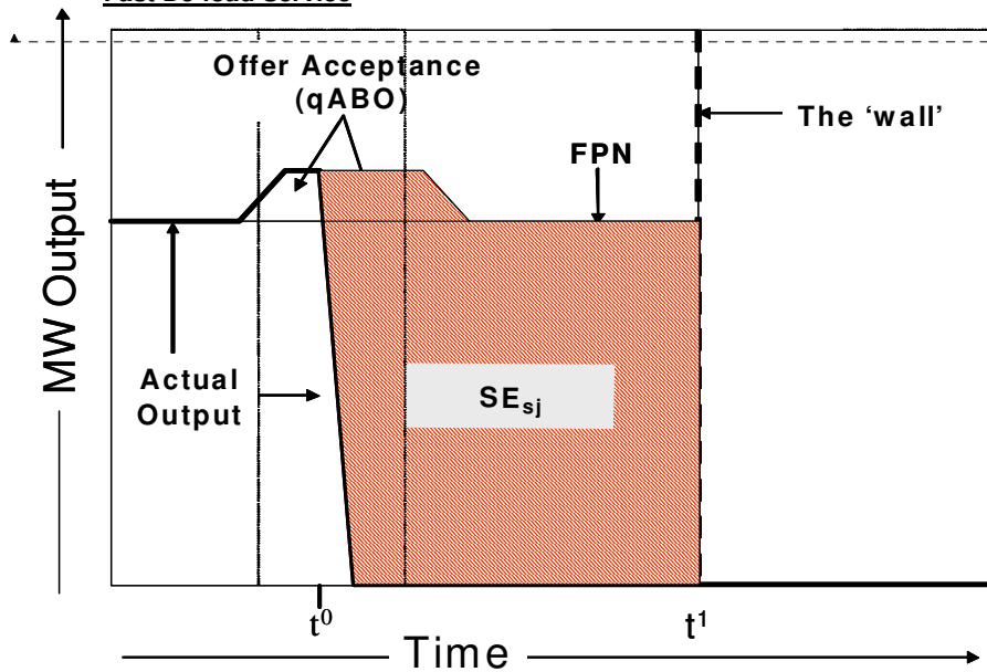
Fig 3a – Graph showing example of SE_{sj} for System to Generator Operational Intertripping Scheme or a Commercial Intertripping Scheme (time delayed) or a Fast De-load Service
