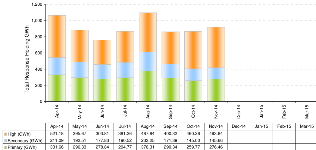
Mandatory Frequency Response Holding
