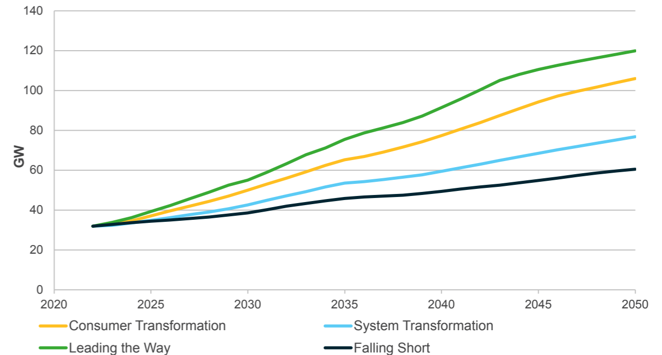
Figure ES.22: Distribution connection generation
