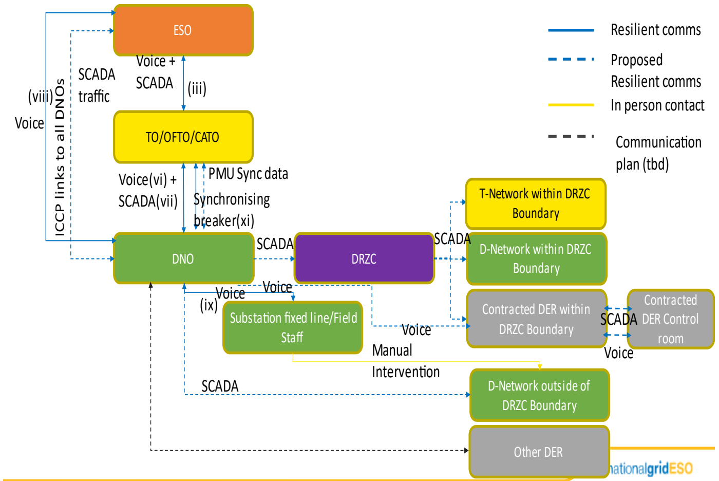
Figure 2: Proposed Distribution Led restoration communication map
