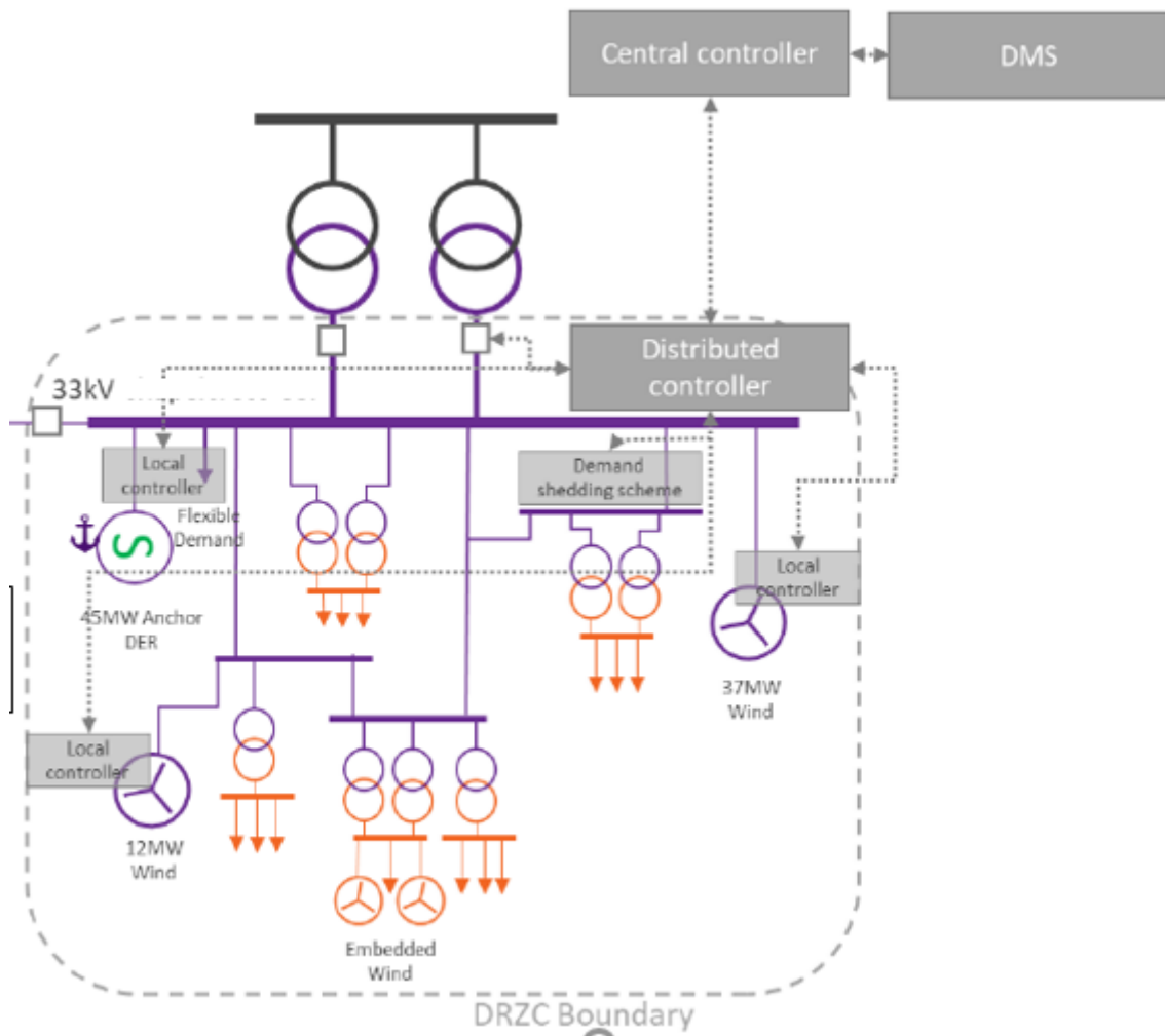
Figure 8: DRZC Schematics
