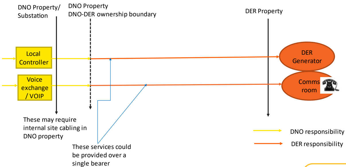
Figure 7: DNO-DER ownership boundary located in DNO property
