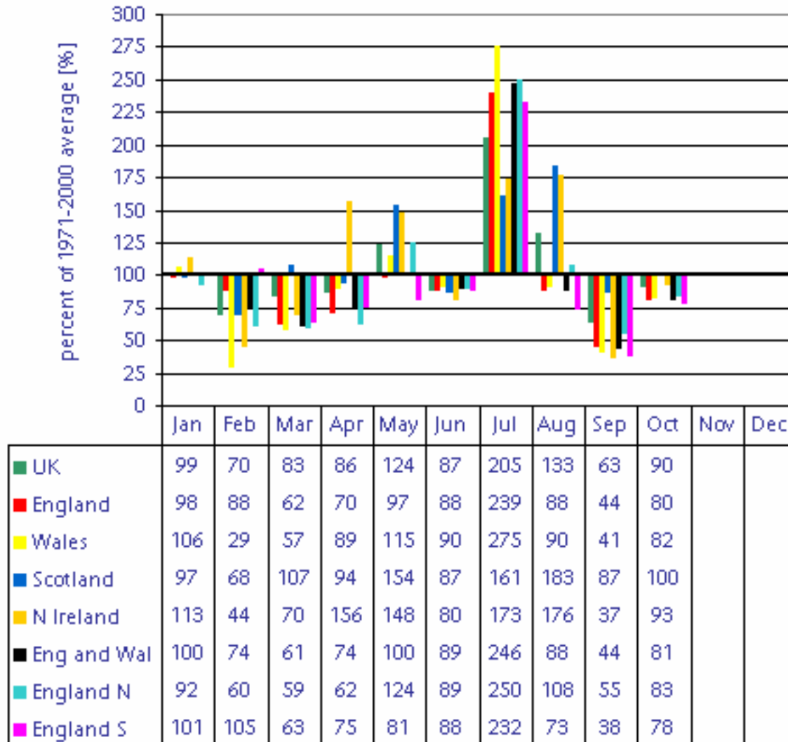
Rainfall (1971-2000) anomalies for 2009
