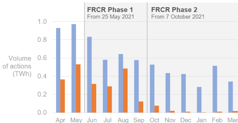
Monthly volume of actions taken to constrain RoCoF risks
