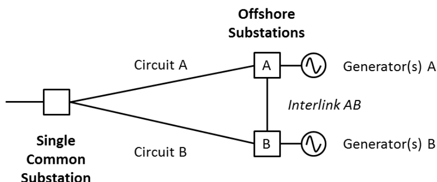
Figure 4: A configuration with two generators and one interlink.
