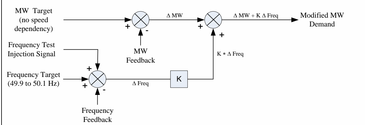
Figure C4 Typical Frequency Test Injection Scheme
