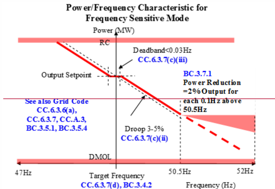
Figure C2 – Frequency Sensitive Mode
