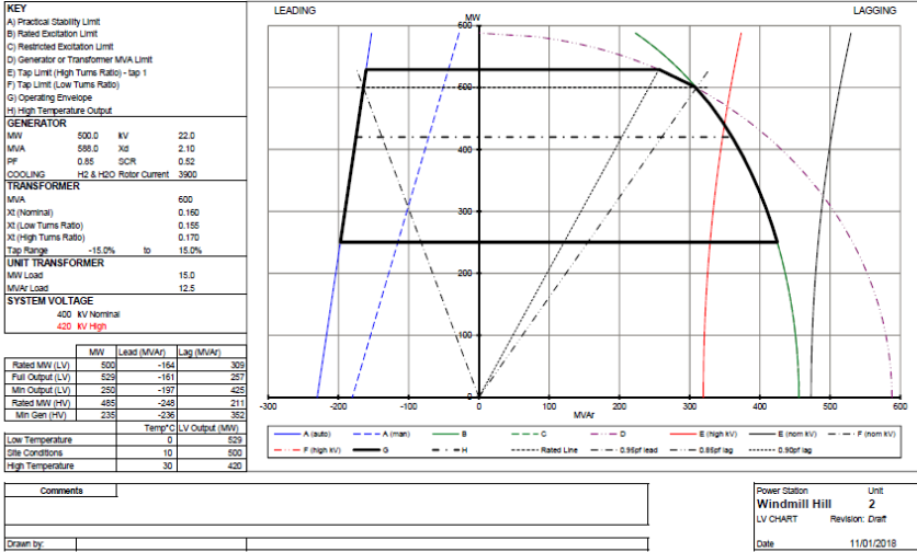
GENERATOR PERFORMANCE CHART
